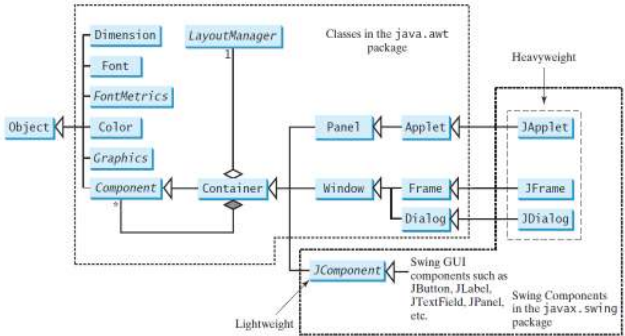
FIGURE 12.1 Java GUI programming utilizes the classes shown in this hierarchical diagram.
